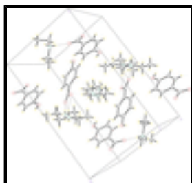
Fig. 2. A view of the hydrogen-bonding patterns in (I). Dashed lines indicate hydrogen bonding.
